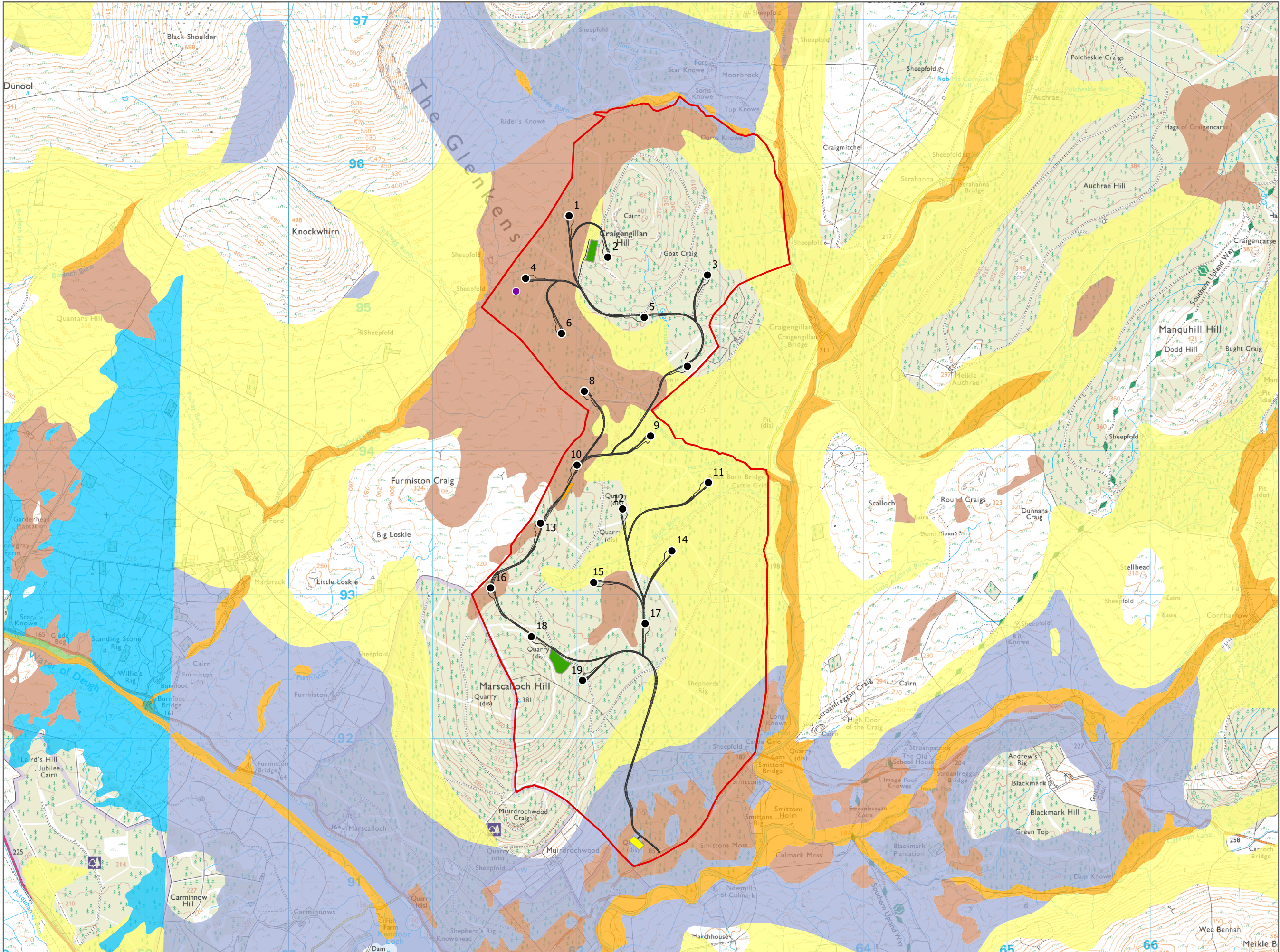
Figure 12.1: Superficial Soils
